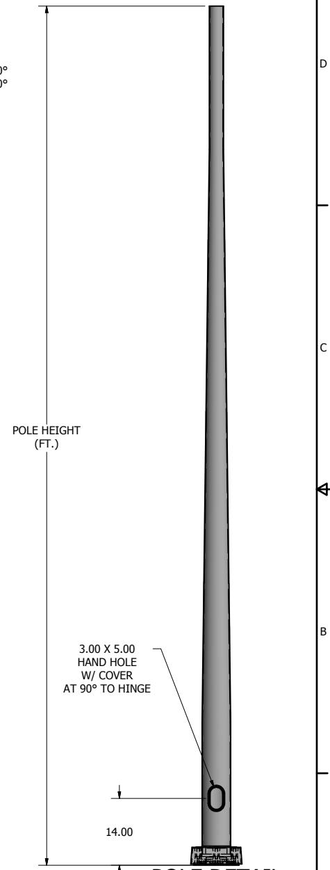
POLE DETAIL
